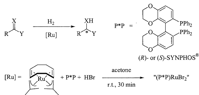
Scheme 6. General procedure for ruthenium-mediated asymmetric hydrogenation reactions using SYNPHOS ®
