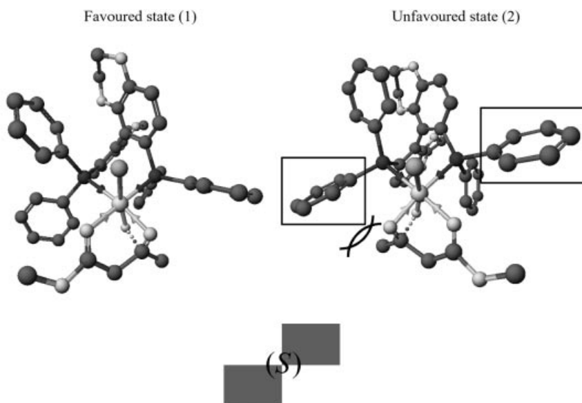
Figure 5. Quadrants diagram for ( S )-SYNPHOS ®
