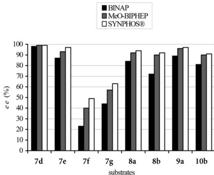
Figure 6. Correlation between \theta and ee in the asymmetric ruthenium-mediated hydrogenation
