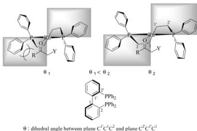
Figure 7. Steric hindrance and dihedral angles
