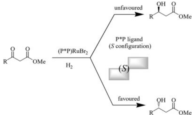
Scheme 9. Sense of enantioselectivity in the asymmetric Ru-catalyzed hydrogenation of \beta -keto esters
