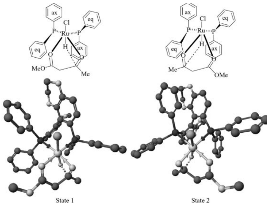
Figure 3. Diastereomeric intermediates {[( S )-SYNPHOS®]RuHCl-CH 3 COCH 2 COOCH 3 } (CAChe MM2 representation)
