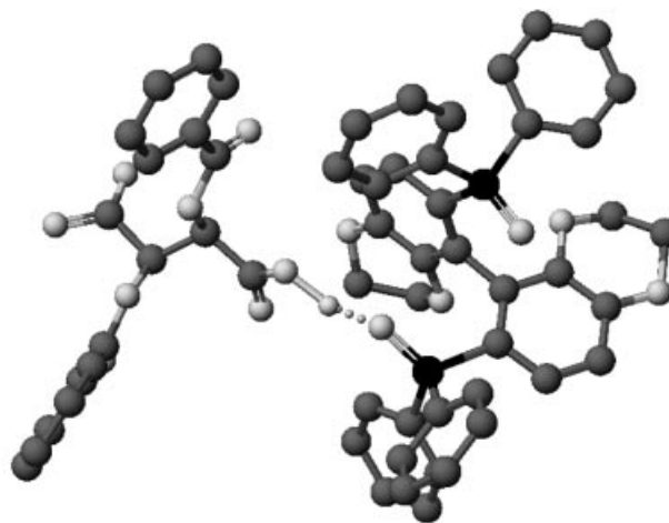
Figure 1. X-ray structure of [(-)-DBTA·( S )-5] (Chem3D representation, H atoms omitted for clarity)
